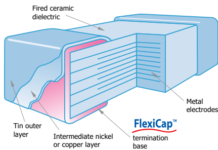
FlexiCap™ MLCC cross section
