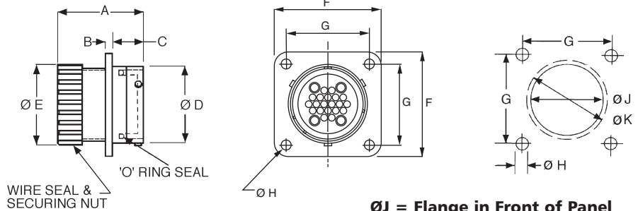
Panel Cutout
