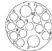
Shell Size 16 2 Power 13 Signal
