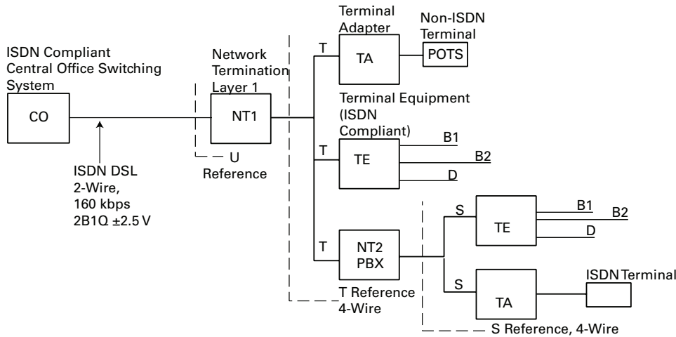
Figure 4.41 ISDN Protection
