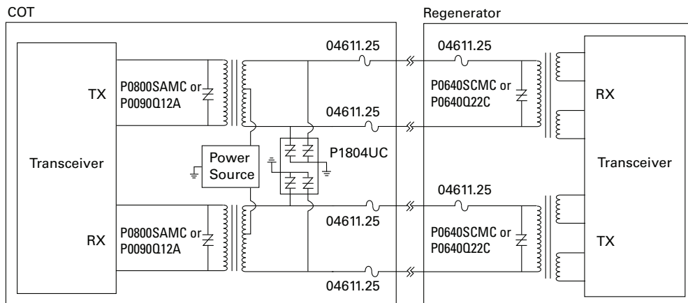
Figure 4.19 T1/E1/J1 Symmetrical Protection
