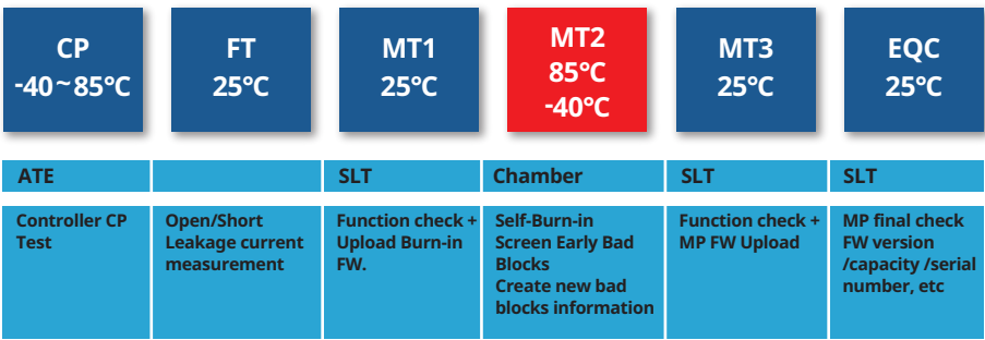
Fig. 4: comprehensive high- and low-temperature test routines are applied to every part shipped to an automotive customer. (Image credit: Silicon Motion)
