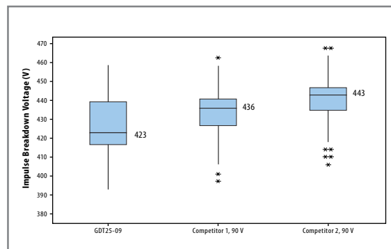
Figure 6 - Impulse Comparison, 1 kV/ \mu s 90 V Models
