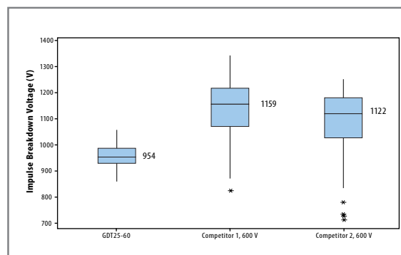
Figure 8 - Impulse Comparison, 1 kV/ \mu s 600 V Models
