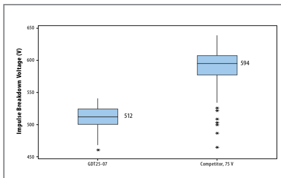
Figure 5 - Impulse Comparison, 1 kV/ \mu s 75 V Models
