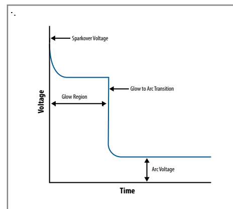
Figure 2 - GDT Voltage Breakdown
