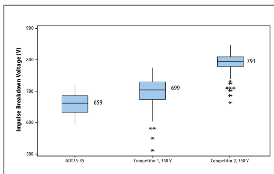
Figure 7 - Impulse Comparison, 1 kV/ \mu s 350 V Models
